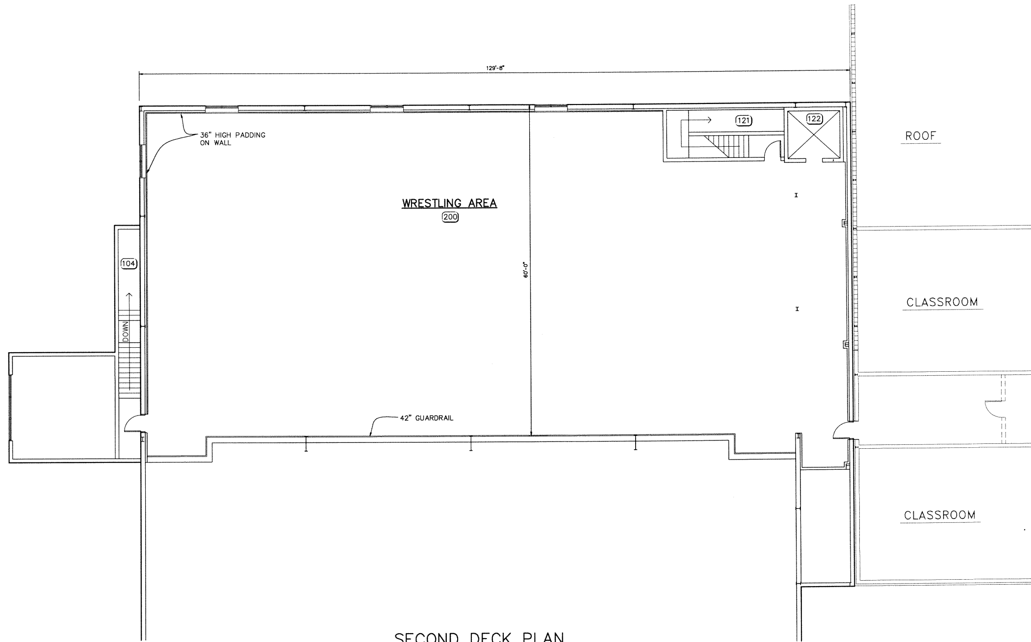
SECOND DECK PLAN 3/32" = 1' - 0"
